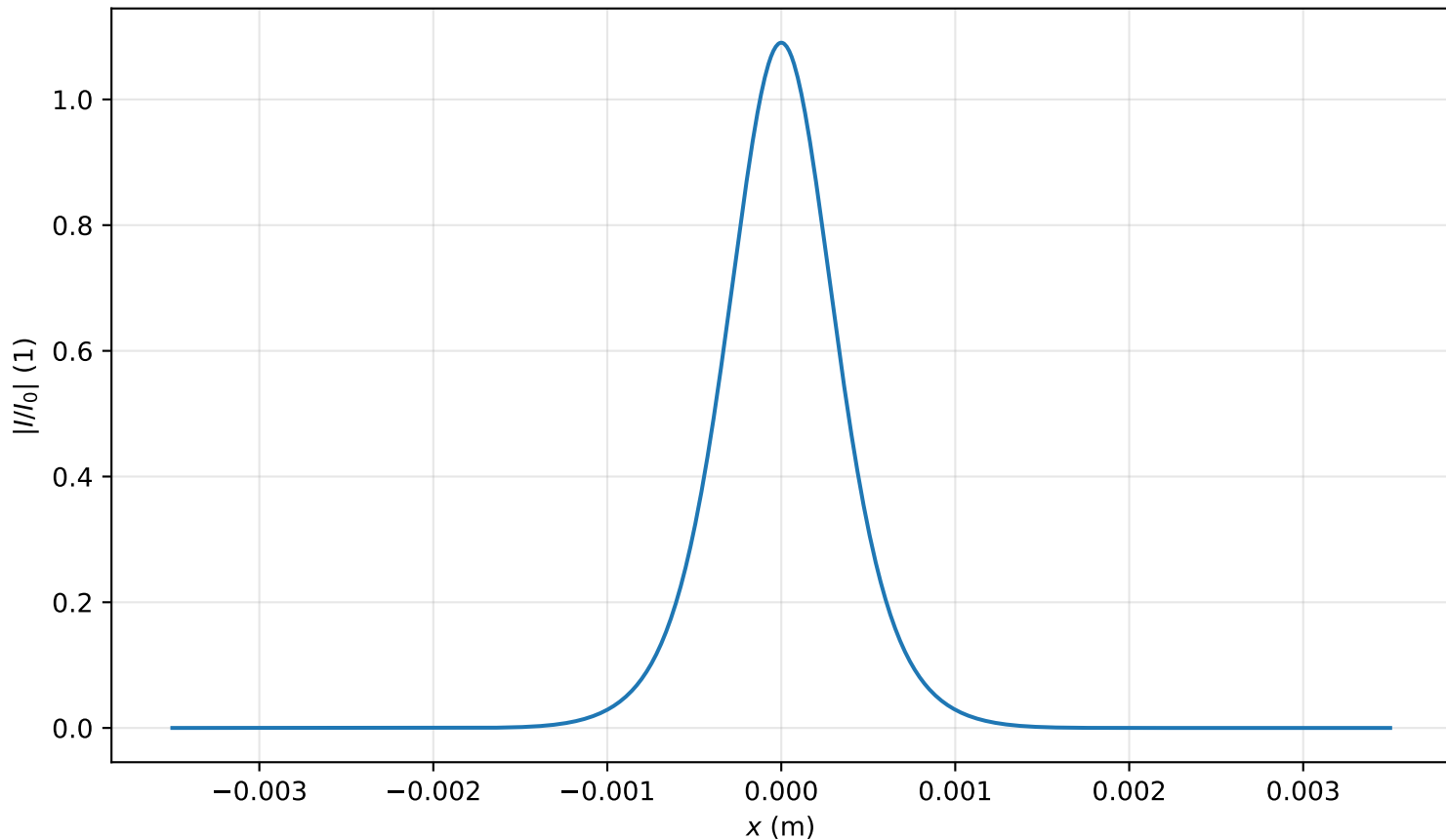
Intensity profile I(x, y = 0, z = 1.353m)/I_0 , P_{in}=0.6P_{cr} , artificial time
